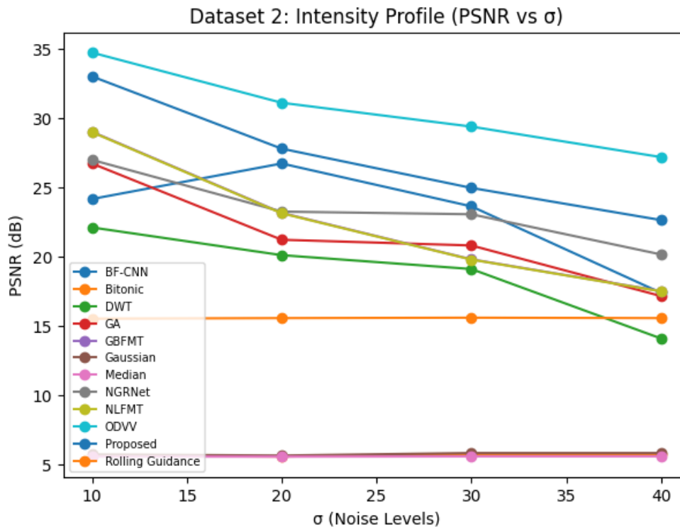
Fig. (18). Intensity profile for dataset 2.
