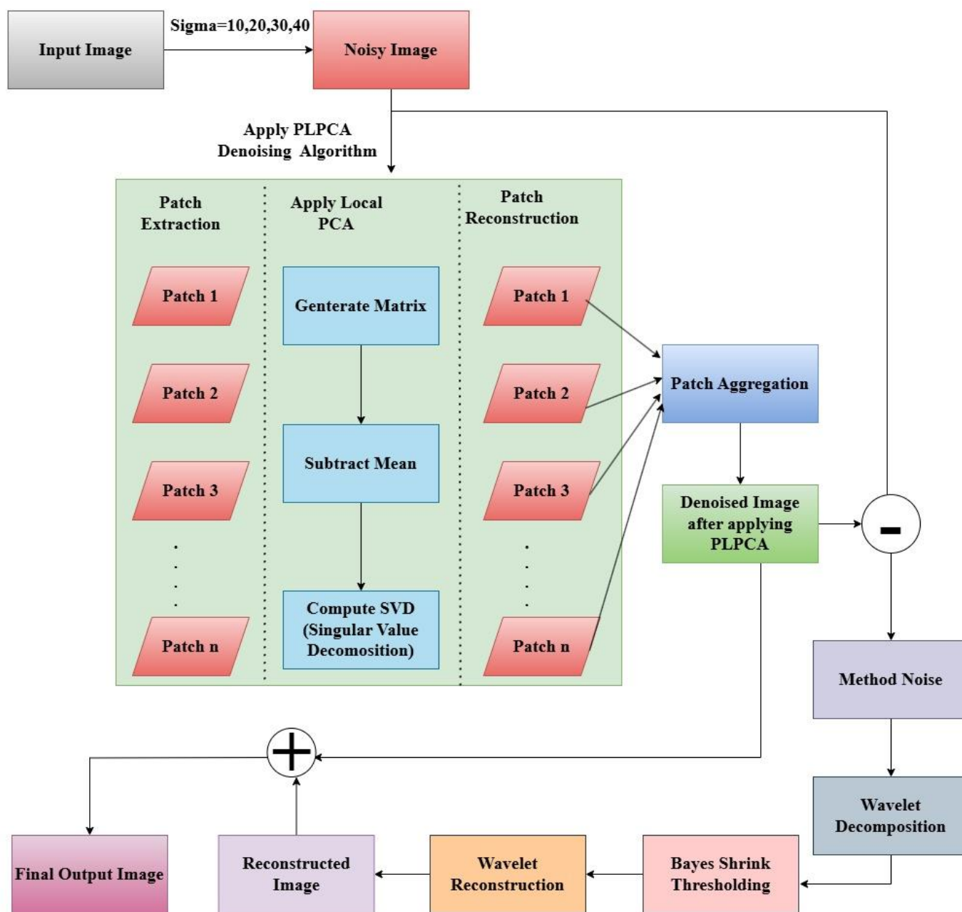
Fig. (2). Proposed methodology for image denoising.
