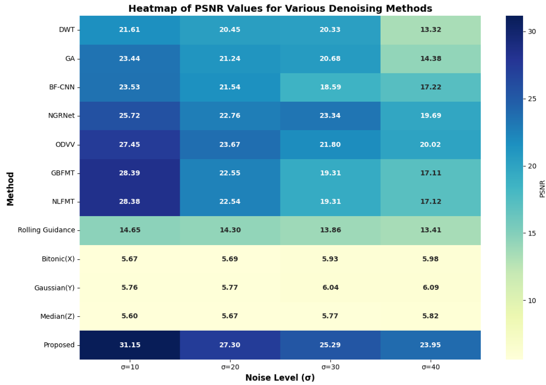
Fig. (11). Heatmap for dataset 1.
