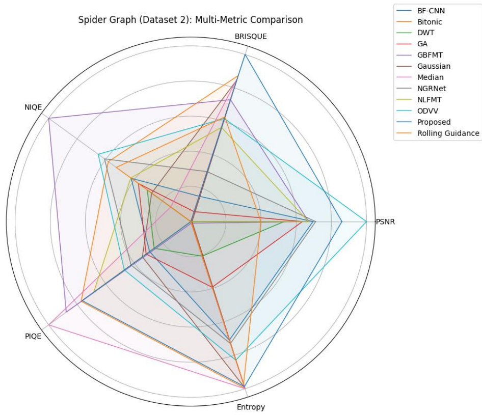
Fig. (16). Spider graph for dataset 2.
