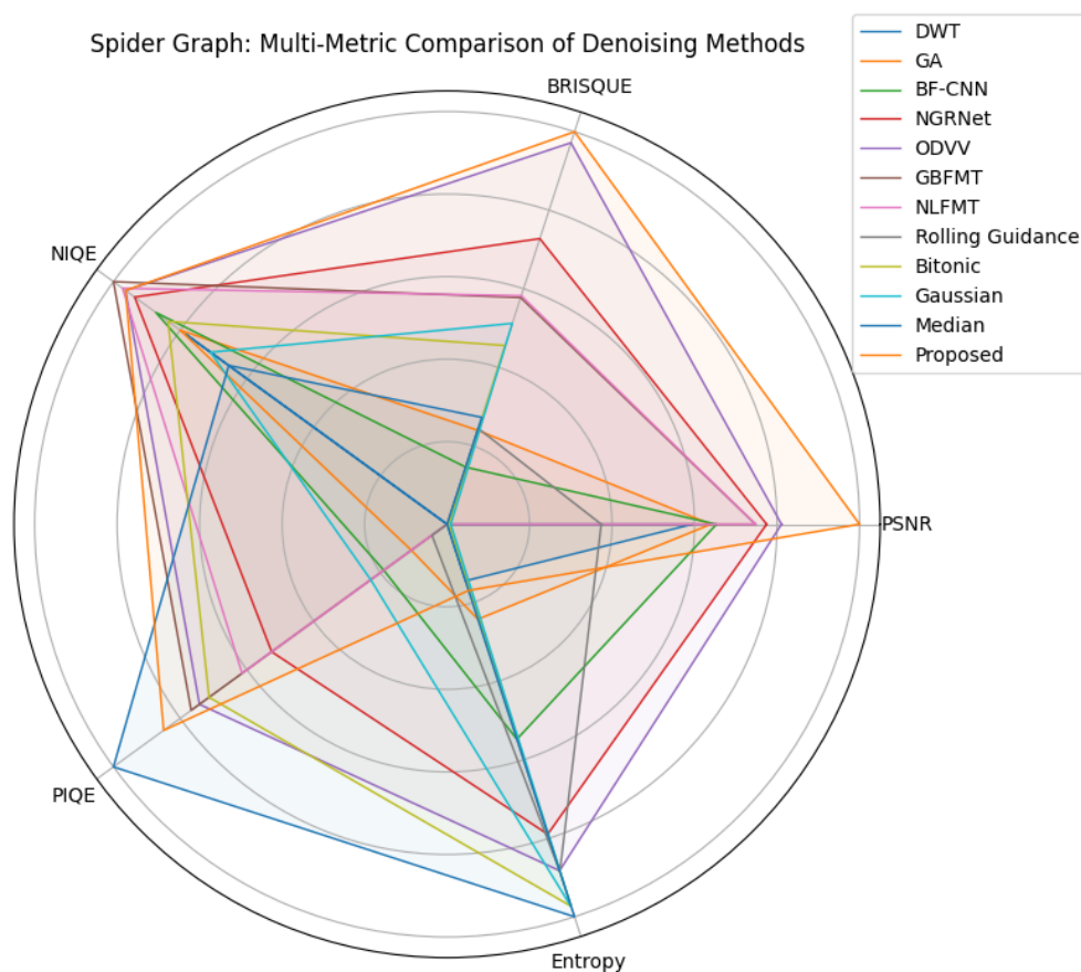
Fig. (15). Spider graph for dataset 1.
