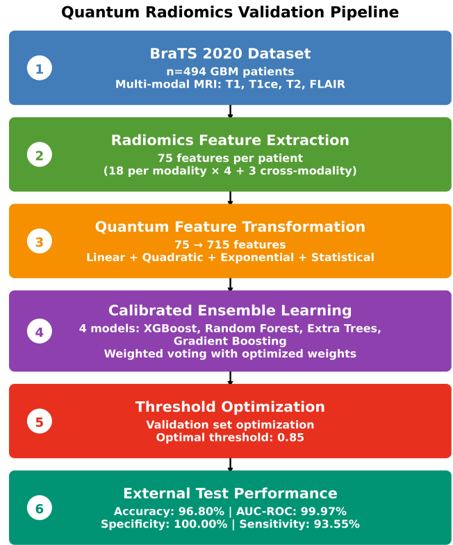
Fig. (4). Complete validation pipeline showing workflow from BraTS 2020 data through radiomics extraction, quantum transformation, ensemble learning, to final test performance.
