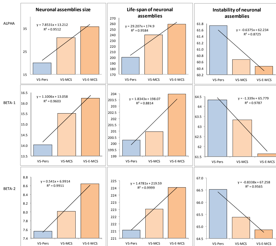
Fig. (2). Features and dynamics of neuronal assemblies (indexed by EEG segment attributes) as a function of clinical outcome 6 years post-injury: Linear regression analysis. Data are averaged across all EEG channels and all 1-minute EEGs within each state. The values of attributes of neuronal assemblies indicated by the Y-axis: size of neuronal assemblies—amplitude within each segment (microvolt); life-span of neuronal assemblies—length of segments (milliseconds); instability of neuronal assemblies—coefficient of amplitude variability within segments (%). Lines in the graphs represent the linear regression equation and R^2 . Abbreviations: Alpha: EEG rhythm 7-13 Hz; Beta-1: EEG rhythm 15-25 Hz; Beta-2: EEG rhythm 25-30 Hz. EEG: electroencephalogram; VS-Pers: patient continues to be in persistent vegetative state 6 years post-injury; VS-MCS: patient continues to be in minimally conscious state 6 years post-injury; VS-E-MCS: patient emerges from minimally conscious state 6 years post-injury.
