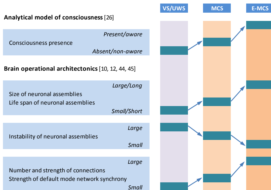
Fig. (1). Schematic presentation of relation of analytical model of consciousness to brain (EEG) operational architectonics parameters. Abbreviations: EEG: electroencephalogram; VS/UWS: vegetative state/unresponsive wakefulness syndrome; MCS: minimally conscious state; E-MCS: emergence from minimally conscious state to full consciousness. Further explanations are provided in the text.
