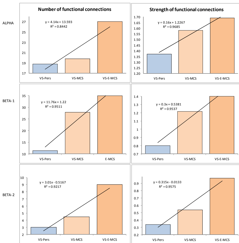
Fig. (3). Operational synchrony among neuronal assemblies (indexed by EEG segments synchronization) as a function of clinical outcome 6 years post-injury: Linear regression analysis. Data are averaged across all pairs of EEG channels and all 1-minute EEGs within each state. The Y-axis presents values of either number (%) or strength of functional connections. Lines in the graphs represent the linear regression equation and R 2 . Abbreviations: Alpha: EEG rhythm 7-13 Hz; Beta-1: EEG rhythm 15-25 Hz; Beta-2: EEG rhythm 25-30 Hz. EEG: electroencephalogram; VS-Pers: patient continues to be in persistent vegetative state 6 years post-injury; VS-MCS: patient continues to be in minimally conscious state 6 years post-injury; VS-E-MCS: patient emerges from minimally conscious state 6 years post-injury.
